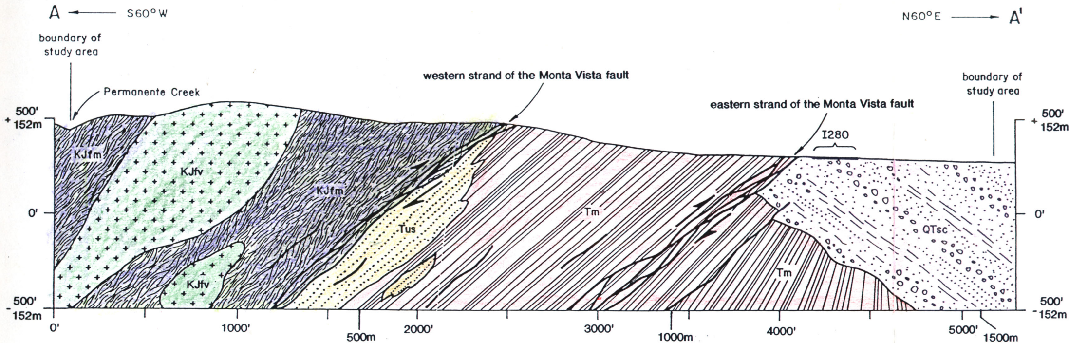
FIGURE 4 GEOLOGIC CROSS SECTION
